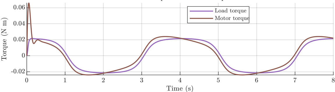
Load Torque and Motor Torque
